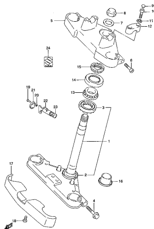
VL250Y 000_042A FRONT FORK BRACKET
