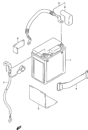
VL250Y 000_020 BATTERY
