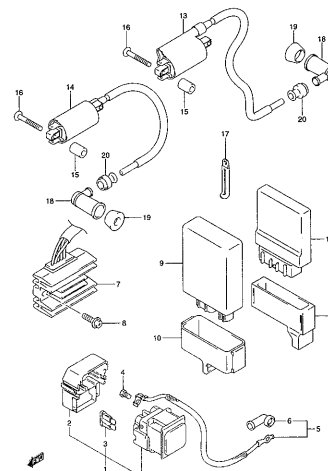
VL250Y 000_021 ELECTRICAL
