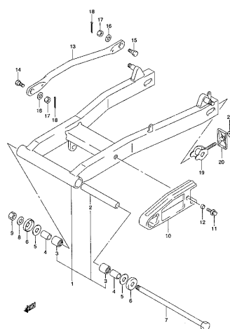
VL250Y 000_046 REAR SWINGING ARM
