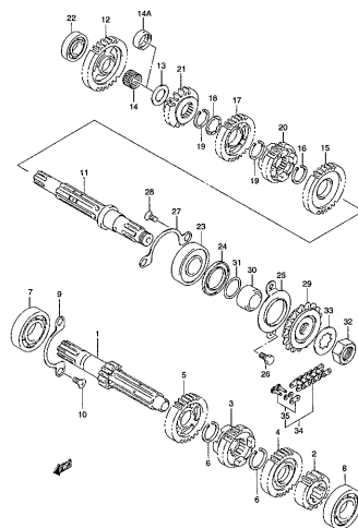
VL250Y 000_016 TRANSMISSION
