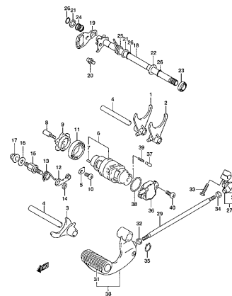
VL250Y 000_017 GEAR SHIFTING
