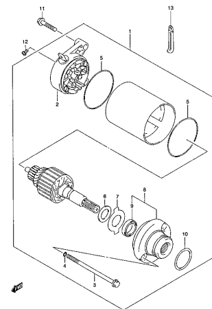
VL250Y 000_018 STARTING MOTOR
