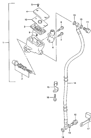
VL250Y 000_045 FRONT MASTER CYLINDER
