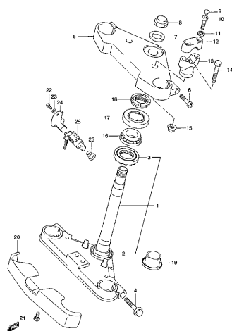
VL250Y 000_042 FRONT FORK BRACKET
