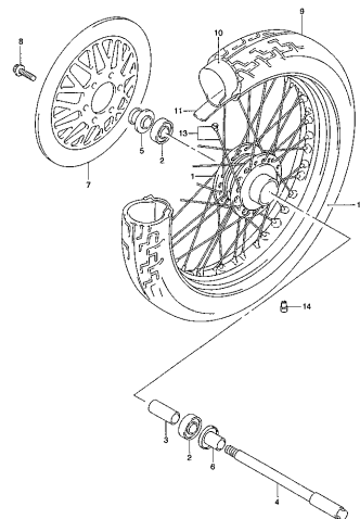
VL250Y 000_043 FRONT WHEEL
