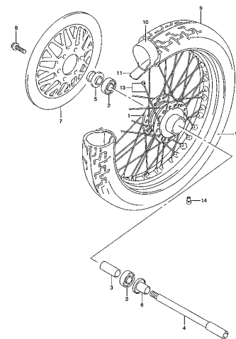
VL250Y 000_043A FRONT WHEEL
