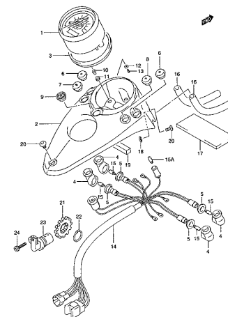
VL250Y 000_022 SPEEDOMETER
