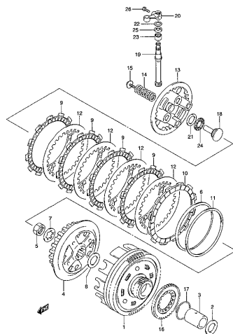
VL250Y 000_015 CLUTCH
