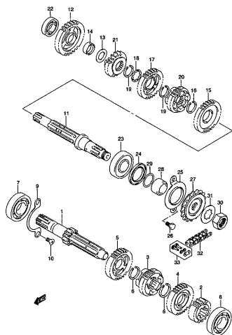
VL250K3 000_017 TRANSMISSION
