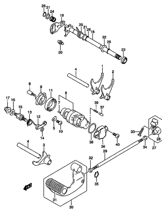
VL250K3 000_018 GEAR SHIFTING
