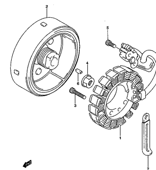
VL250K3 000_020 MAGNETO
