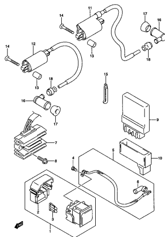
VL250K3 000_022 ELECTRICAL
