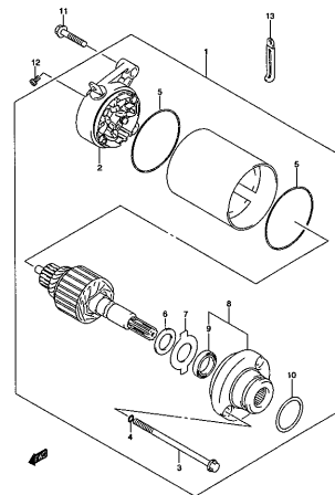
VL250K3 000_019 STARTING MOTOR
