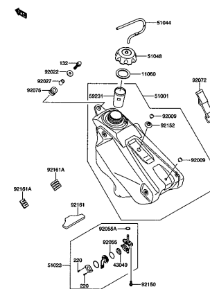
RM-Z250K4 000_040 FUEL TANK
