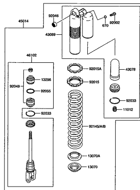
RM-Z250K4 000_033 SHOCK ABSORBER
