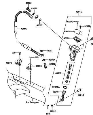
RM-Z250K4 000_036 REAR MASTER CYLINDER
