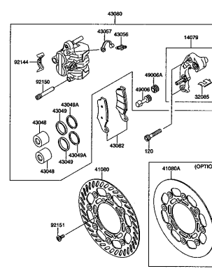
RM-Z250K4 000_035 FRONT BRAKE
