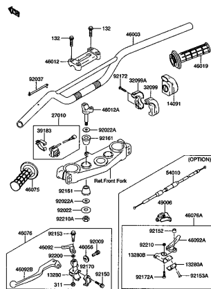
RM-Z250K4 000_038 HANDLEBAR
