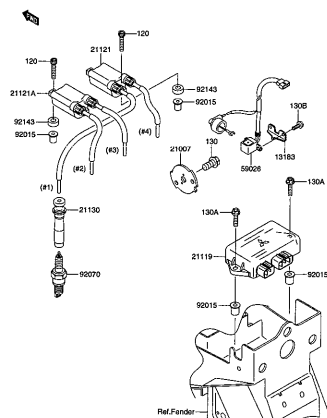
GSX250FXTK3 000_021 IGNITION SYSTEM
