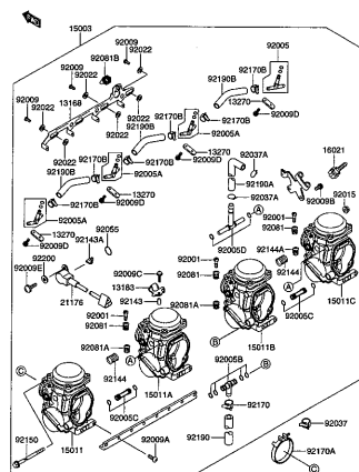
GSX250FXTK3 000_017 CARBURETOR
