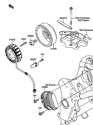
GSX250FXTK3 000_020 GENERATOR
