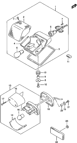
DR250RXKX 000_009 REAR COMBINATION LAMP
