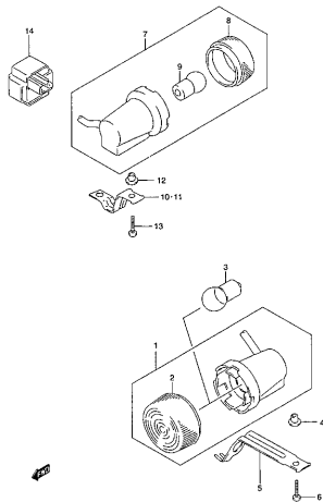
DR250RXKX 000_027 TURN SIGNAL LAMP
